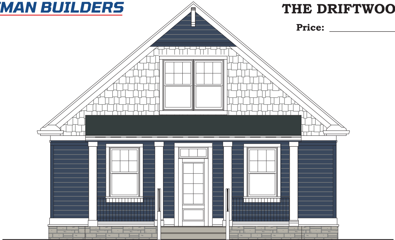
FRONT ELEVATION BH212
