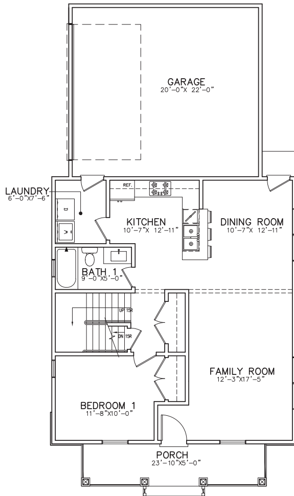
FIRST FLOOR 911 SF W/ BASEMENT
