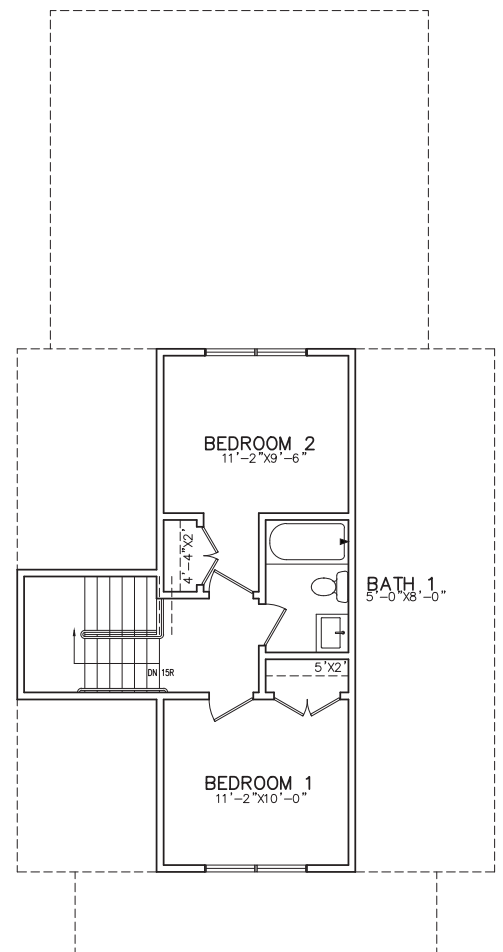
SECOND FLOOR 378 SF
