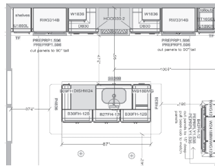
OPTIONAL KITCHEN LAYOUT
