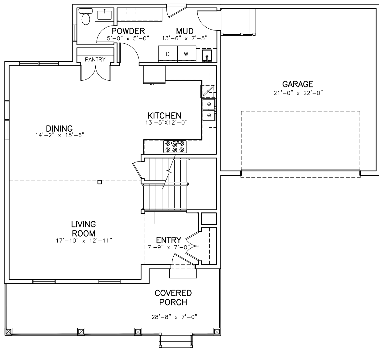
FIRST FLOOR 1013 SF GARAGE 500 SF
